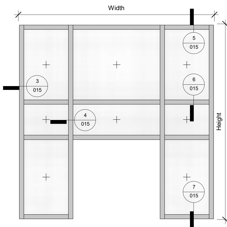
1 Elevation Front 1 : 20
